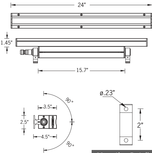
Mounting Detail
